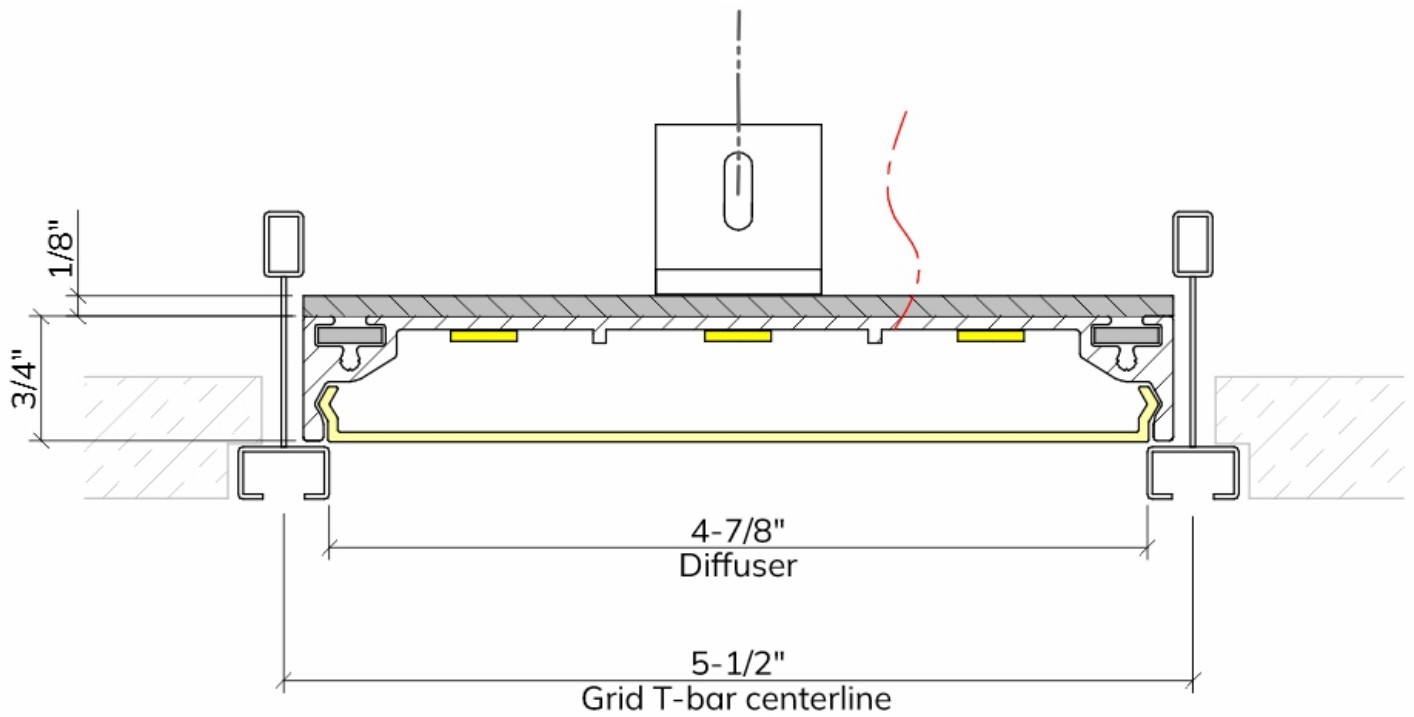
9/16" T-slotted grid bar
